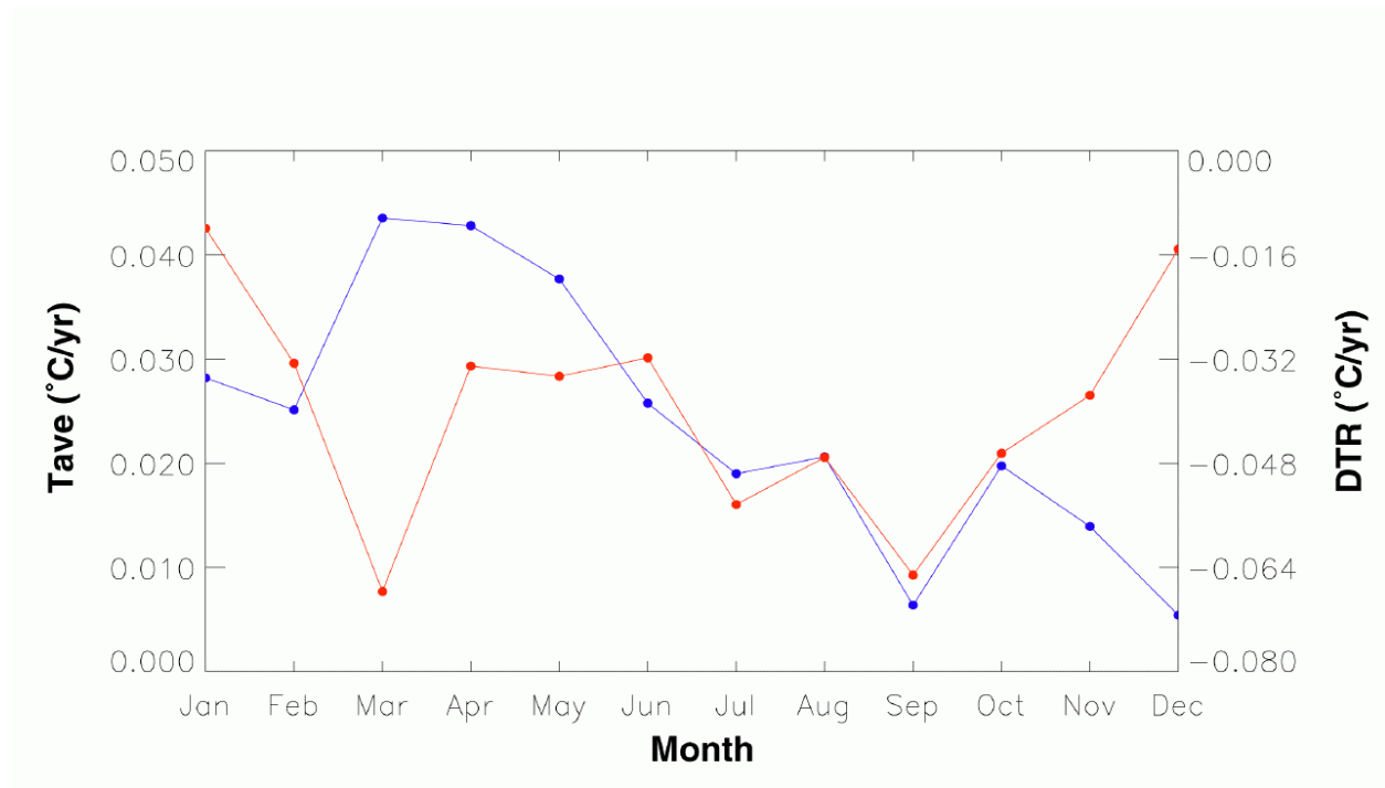
Figure 4. Napa/Sonoma monthly Tave and DTR trends from 1951-1997. Tave trends (blue line and circles) were significant at the 5% level in all months except December. DTR trends (red line and circles) were significant in March, May, July, August, September, and October. Tmax declined during summer months and increased during spring, but changes were not significant in any month. Spring warming and a decline in summer DTR, consistent with global trends, are favorable for winegrape cultivation (Table 1). The large DTR decline in March was accompanied by the highest monthly increases in nighttime cloud cover (18%/47 yr, p=0.010 ), Tdew (2.73°C/47 yr, p<0.001 ), and Tmin (3.62°C/47 yr, p<0.001 ) along with a small but insignificant increase in precipitation.
