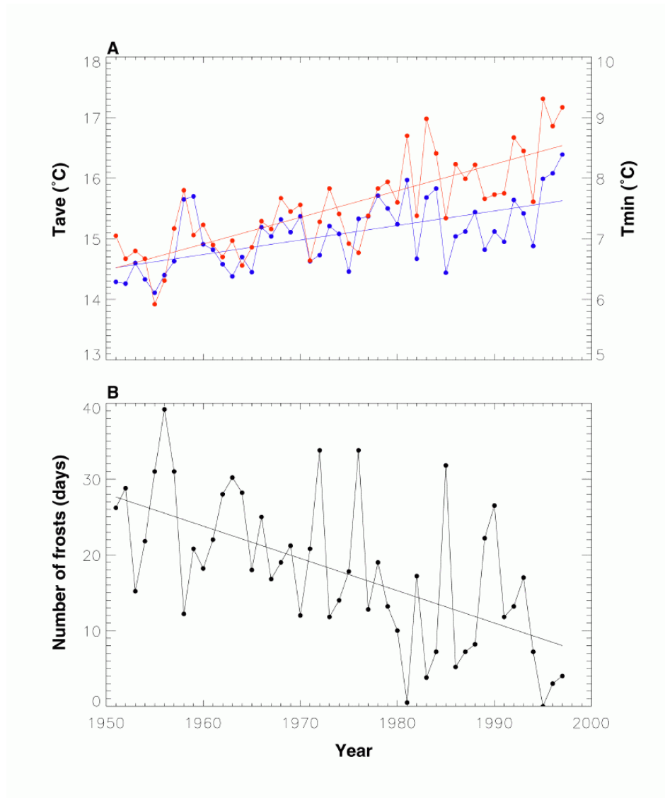
Figure 3. Napa/Sonoma climatic changes. (A) Tave increased 1.13^{\circ}\text{C}/47 yr ( p < 0.001 , blue line and circles) with nearly all warming caused by increasing Tmin ( 2.06^{\circ}\text{C}/47 yr, p < 0.001 , red line and circles). Consequently, DTR declined by 1.87^{\circ}\text{C}/47 yr ( p < 0.001 ). Contribution of Tmin to Tave increase is higher than in global trends. (B) Napa/Sonoma frost decreased 71\%/47 yr ( p < 0.001 ). If current trends continue, Napa/Sonoma will become a frost-free climate, indicating a fundamental shift in ecosystem function.
