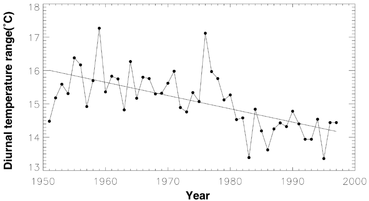
Figure 8 (supl). Annual average DTR trends. Asymmetric warming led to a 1.87°C/47 yr compression of the DTR. Temperature variability and temperature extremes, as measured by Gladstones' temperature variability index (TVI) (8), are related to wine quality. Low TVIs favor high-quality wines. In Napa/Sonoma, the TVI declined from 36.1 in 1951 to 31.4 in 1997. TVI values under 30 indicate that any variety of table wine may be produced. Even within a vineyard, sites with higher T min and low DTR as a result of soils or topography are regularly associated with high quality wines (1). TVI = \sum ((TD_{max} - TD_{min}) + (TM_{max} - TM_{min})) , where TD and TM represent daily and monthly values between March and October.
