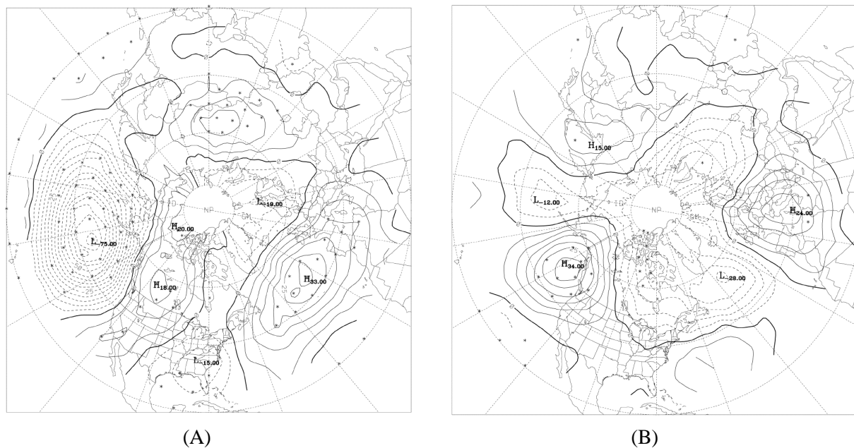
Figure 11 (supl). Winter anomalies of 700 mb pressure heights (m) (11) for high and low frost years in Napa-Sonoma. We calculated the average number of annual frosts and divided the 1951-1997 dataset into above and below average scenarios. For the ten most extreme years within each scenario, we then calculated the composite 700 mb pressure patterns. Winters with low frost occurrence ( A ) are dominated by Pacific low pressure systems while winters with high frost occurrence ( B ) are dominated by Pacific high pressure systems. Since 1976, low pressure systems have become more frequent (12) bringing warm and moist southwesterly winds over the California coast.
