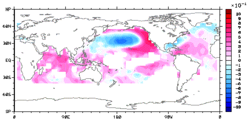
Figure 10 (supl). Correlations between coastal California Tave and SSTs (11) during winter (1946-1998) at each 5° x 5° grid cell. The positive relation between coastal land temperatures and near-coast SSTs suggests a strong maritime influence over the wine producing areas. Warmer winter SSTs, because of their persistence, also lead to warmer spring temperatures. This suggests that given winter SSTs, reasonable prediction of next-year wine quality may be possible. Warmer winter SSTs, on average, lead to higher quality wines from coastal California.
